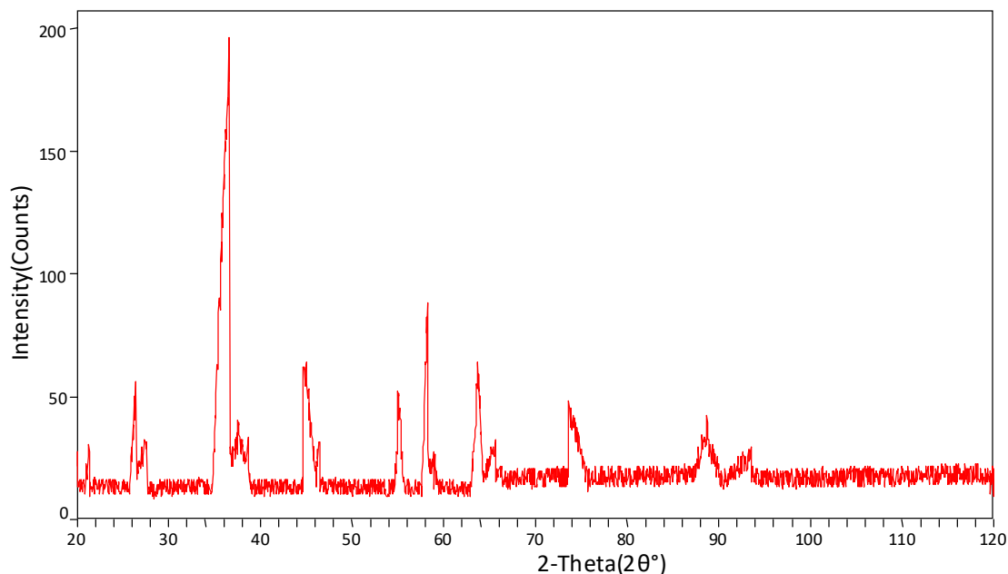
Fig.1: XRD of compound \text{Li}_{0.5}\text{Fe}_{2.5}\text{Al}_8\text{Co}_2\text{O}_{19}
